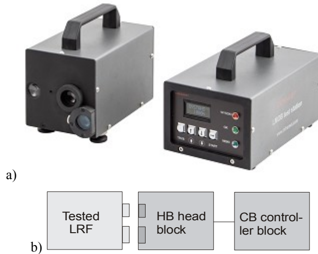
Fig. 1. LMOB test system: a) photo, b) block diagram
