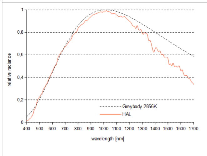
Fig.2. Relative spectrum of SEM1 light source
